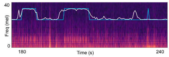
Fig. 7. Mel spectrum of a train signal with superimposed reference annotations (blue) and model output (white). The model correctly labels the longer signals, but overlooks a very short signal and also makes a false positive error. (For interpretation of the references to color in this figure legend, the reader is referred to the web version of this article.)
