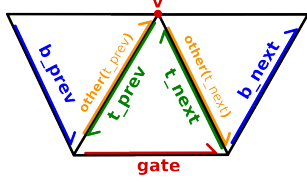
Figure 1: The half-edge data structure used in Edgebreaker.
