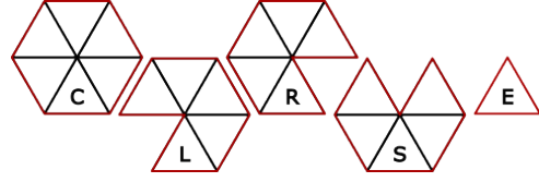
Figure 2: Basic Edgebreaker operations. Red lines represent the boundary of the remaining mesh.
