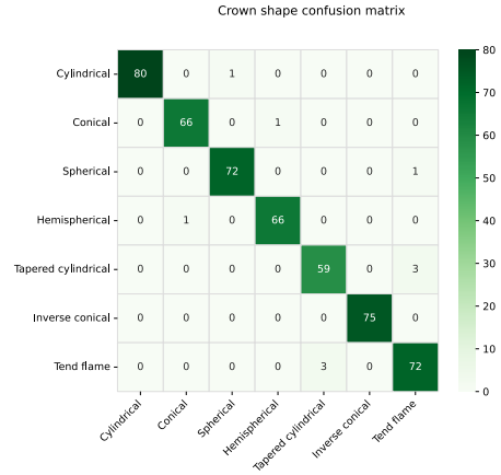
Figure 2: Confusion matrix for classification parameter (crown shape) on the test set. Rows represent the true labels while columns represent the predicted labels.
