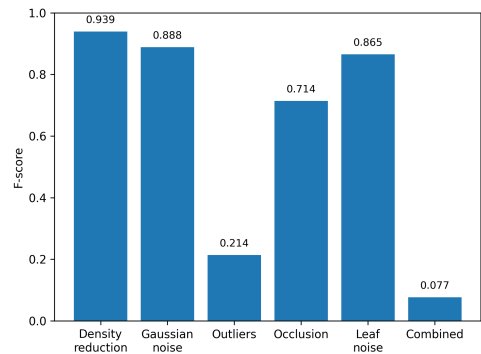
Figure 1: Average F1-score for the most severe degradation level.
