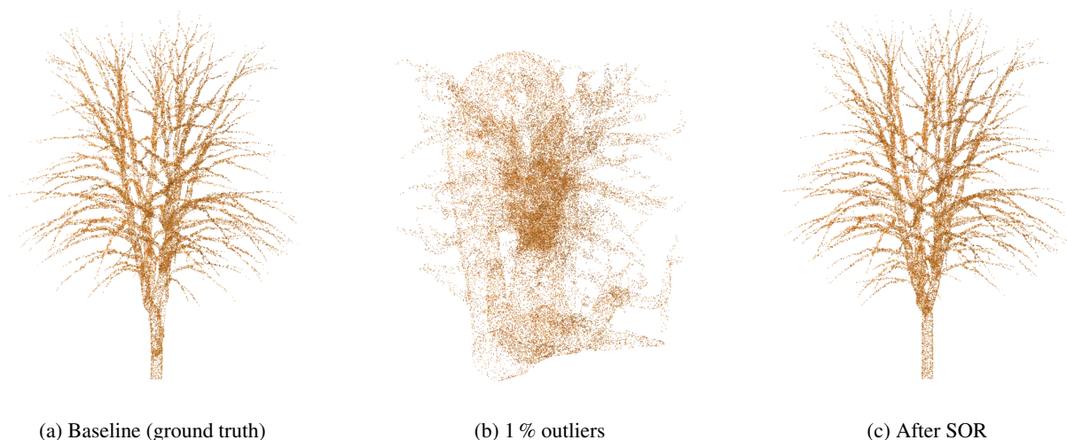
Figure 2: Representative reconstruction results for Tree 3. 1 % isolated outliers cause phantom branches that collapse the skeleton (b), but SOR preprocessing almost fully restores the baseline quality (c).
