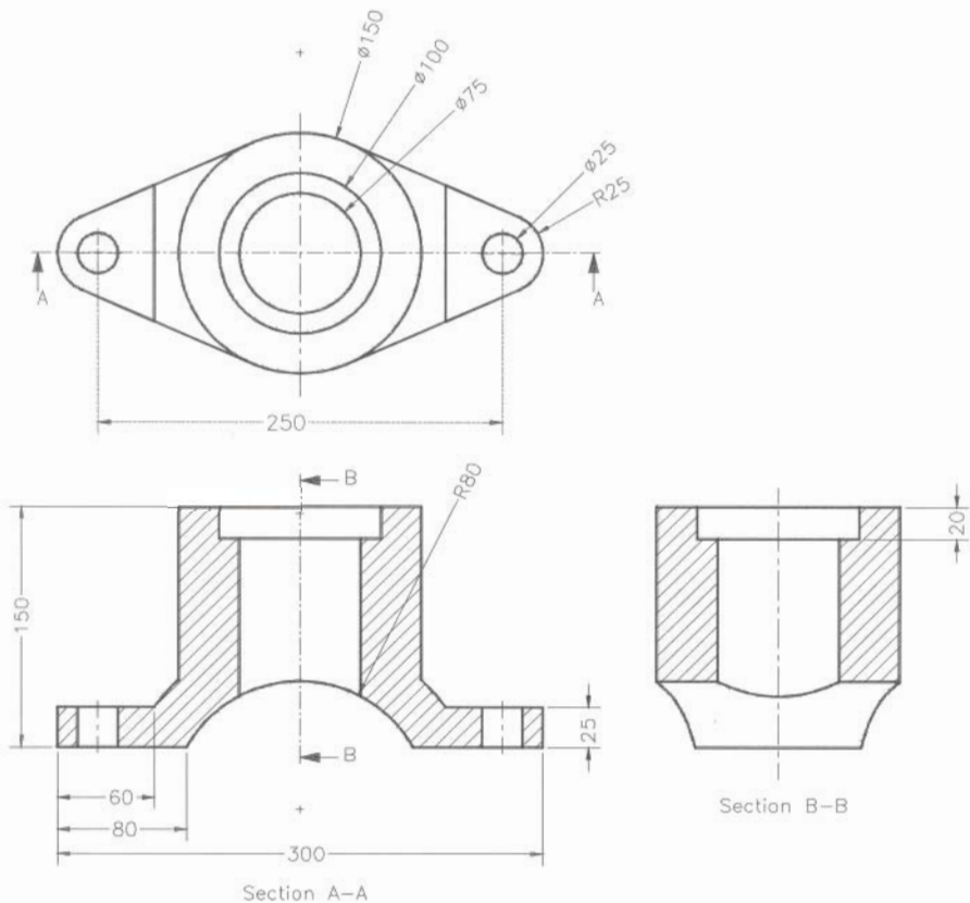
Figure 5-104 Top view, sectioned front view, and sectioned right view of the model
