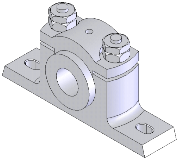
Figure 10-81 Plummer Block assembly
