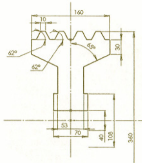
Figure 3-73 Sketch for Exercise 1
